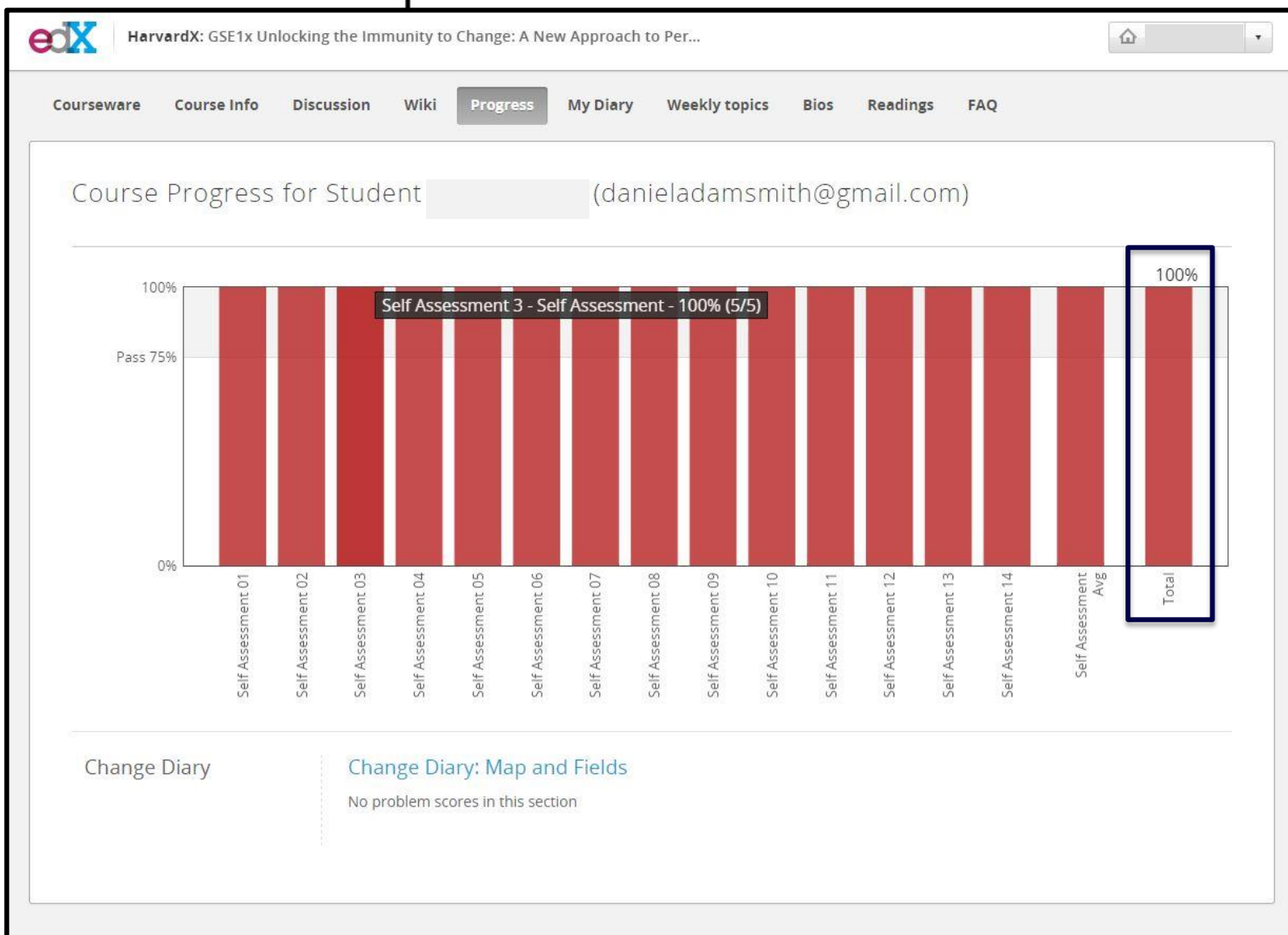
Scoring - Example
